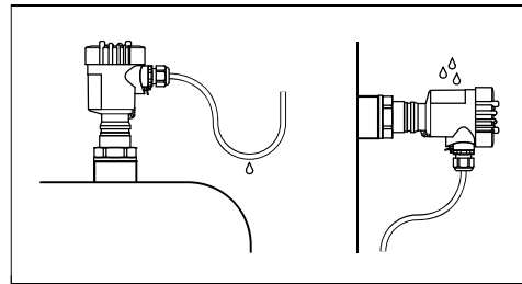
Fig. 9: Measures against moisture penetration
