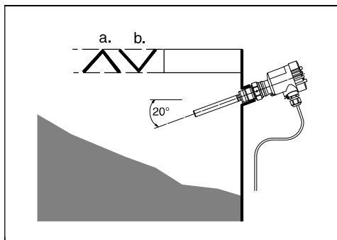
Fig. 10: Horizontal mounting
